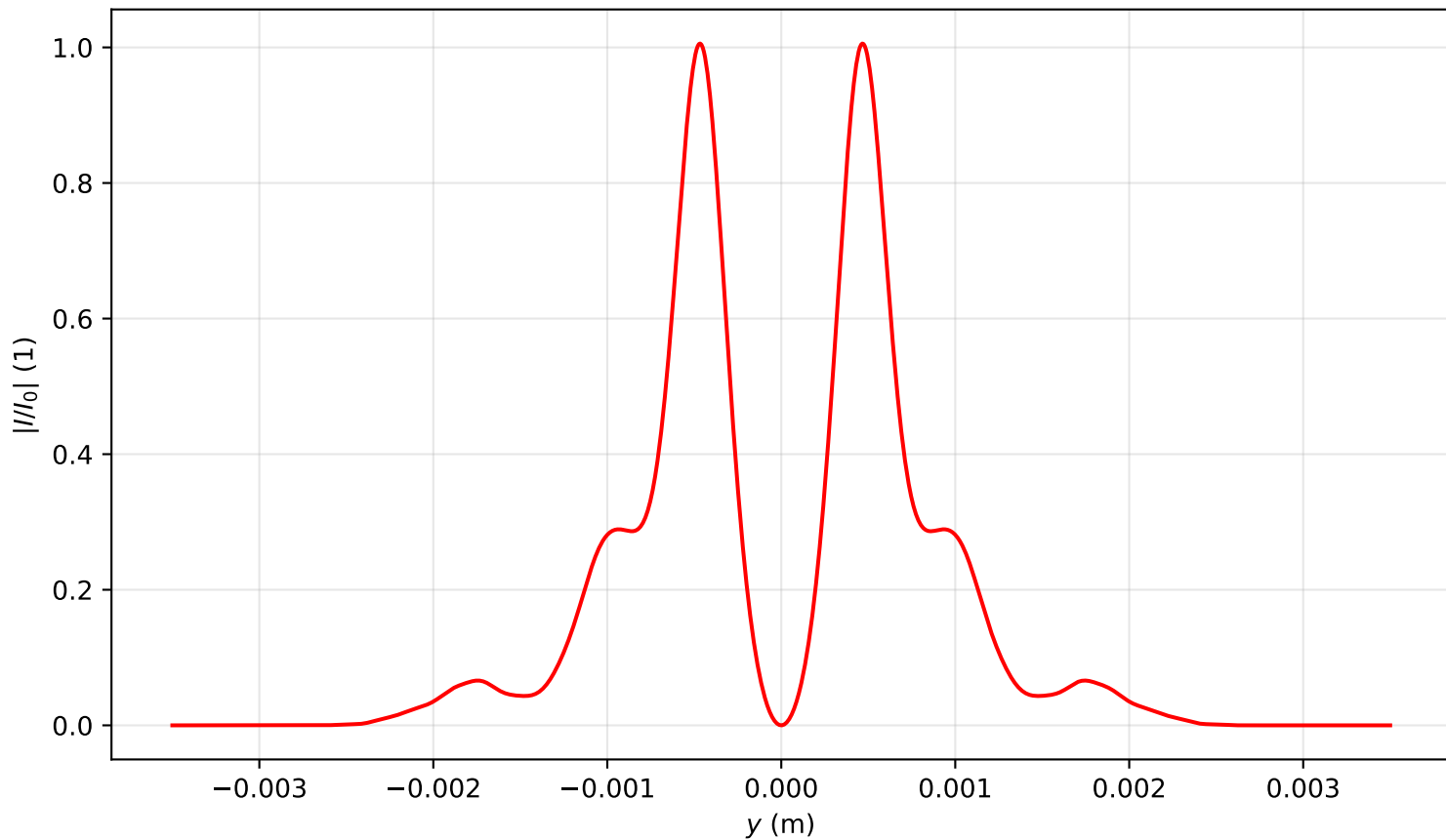
Intensity profile I(x=0, y, z=1.990)/I_0 , P_{in}=6.0P_{cr} , artificial time
